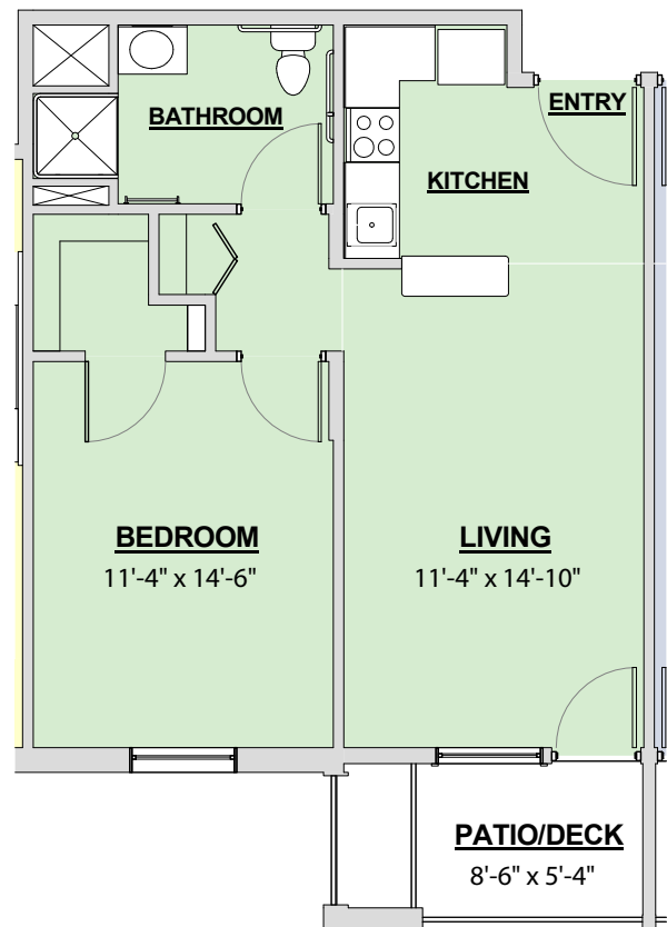
Rosewood II (1 Bedroom w/ Balcony) 636 sq. ft.
